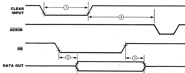
Figure 47. Port 2 Side Operation
