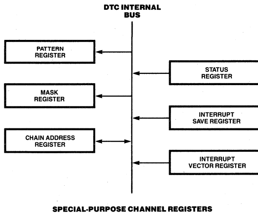
Figure 6. Channel-Level Registers
