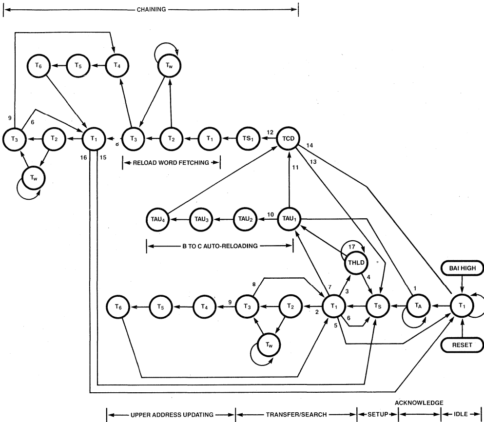
Figure A-12. Z8516/Z9516 State Diagram
