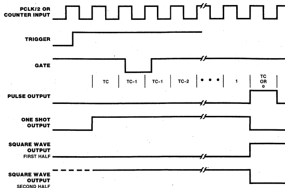
Figure 10. Counter/Timer Waveforms
