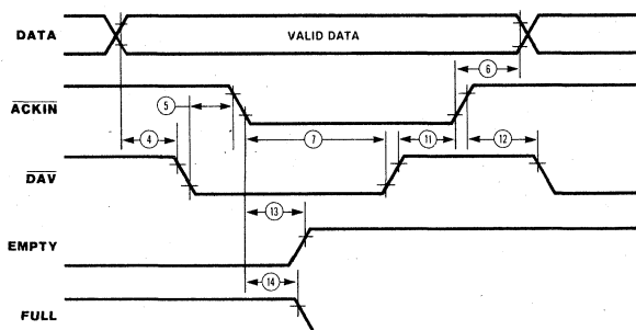
Figure 48. 2-Wire Handshake (Port 2 Side Only) Output
