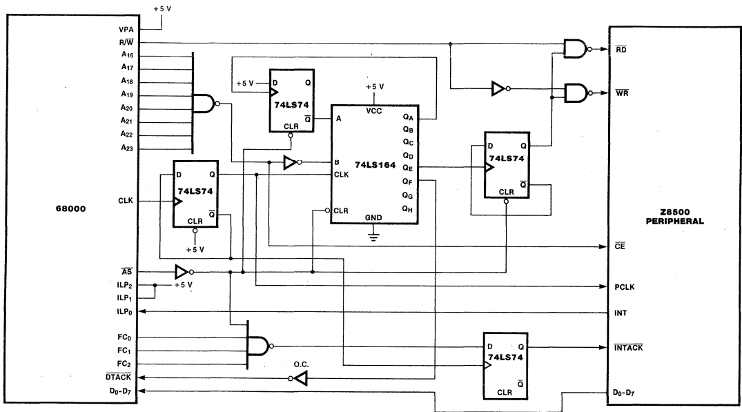
Figure 7. Hardware Diagram for DTACK Interface
