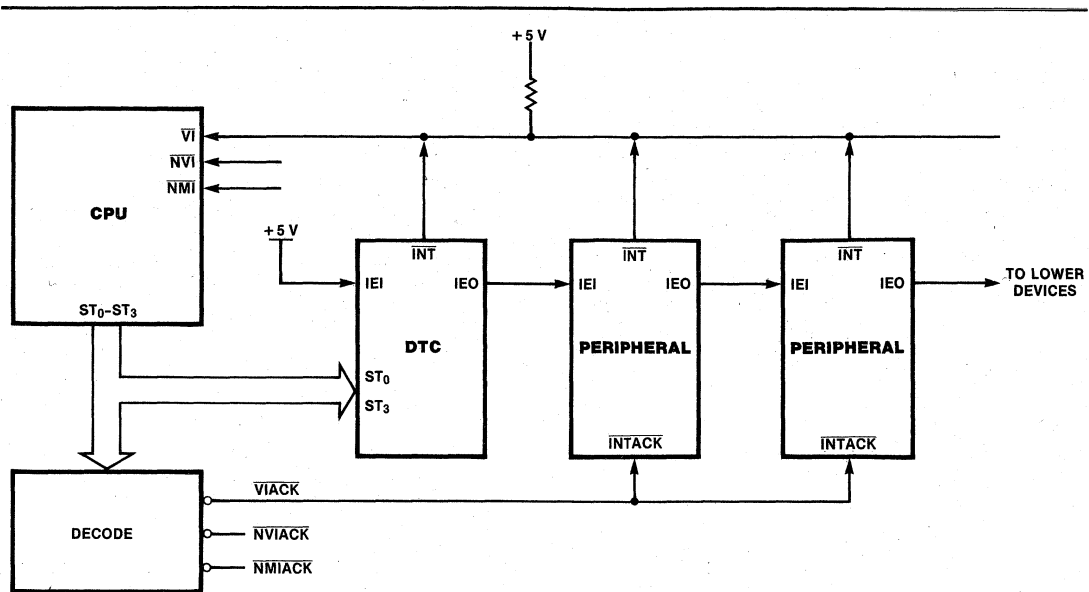
Figure 5. Interrupt Daisy Chain
