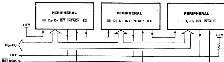
Figure 7. Interrupt Schedule
