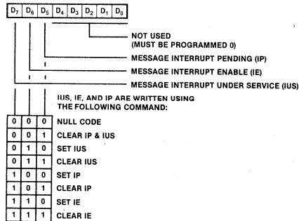
Figure 27. Interrupt Status Registers
