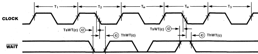
Figure 35. WAIT Timing
