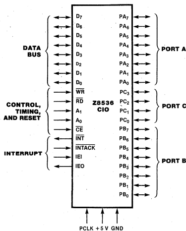
Figure 1. Pin Functions
