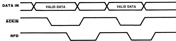
Figure 4. Two-Wire Interlocked Handshake Timing (input)
