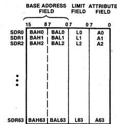
Figure 5. Segment Descriptor Registers
