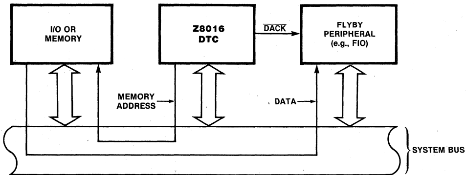
Figure 3. Configuration of a Flyby Transaction
