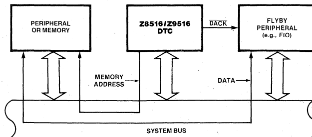
Figure 21. Flyby Transaction
