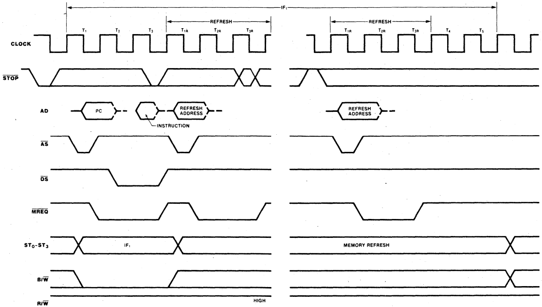
Figure 16. Stop Timing
