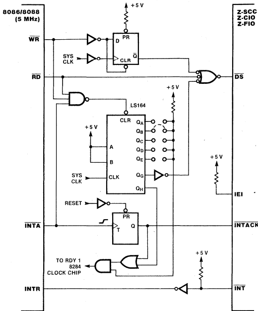
Figure 9. Interrupt Acknowledge Circuit
