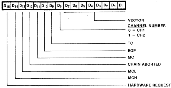
Figure A6. Interrupt Save Registers
