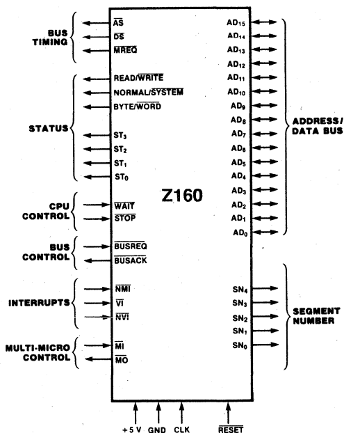
Figure 1. Z160 CPU Pin Functions
