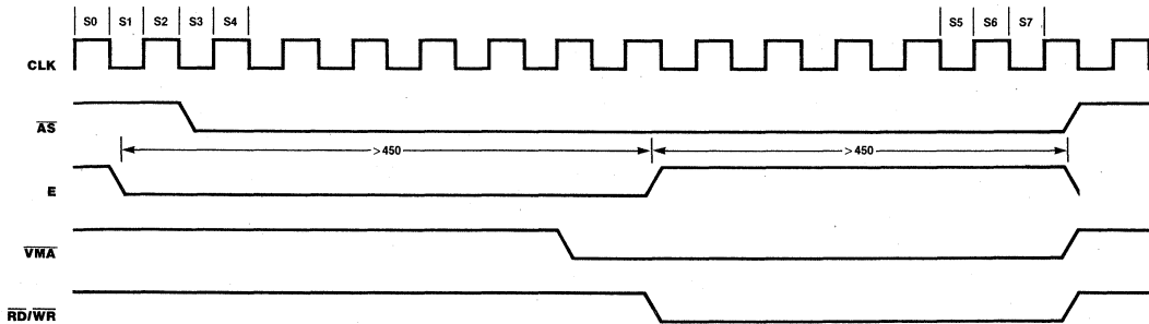
Figure 5. \overline{VPA} Cycle Timing
