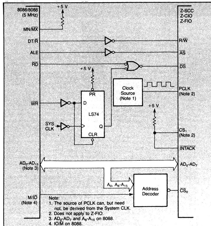
Figure 2: Interface Logic.
