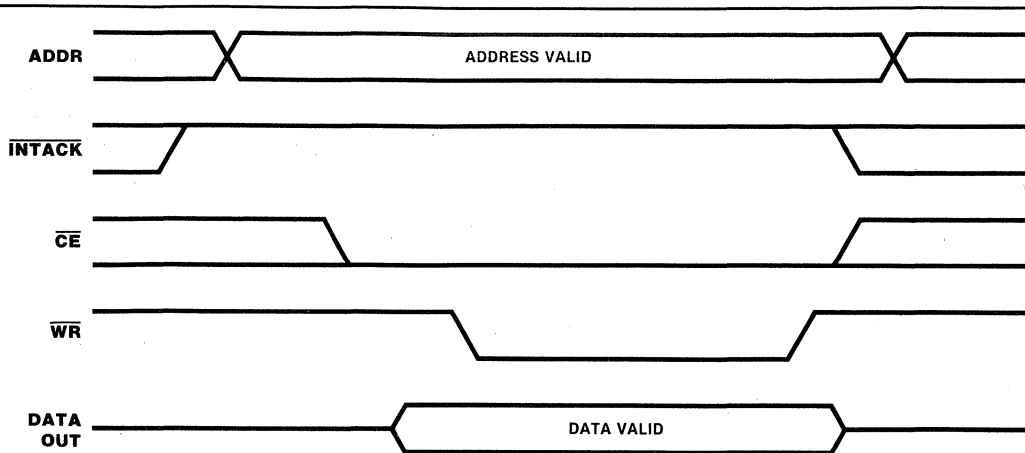
Figure 2. Z8500 Peripheral I/O Write Cycle Timing
