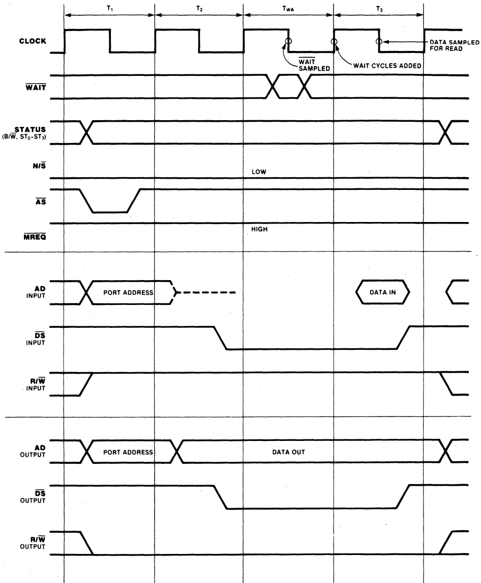
Figure 13. Input/Output Timing
