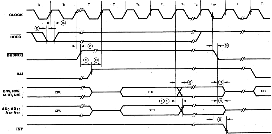
Figure 30. Bus Exchange Timing
