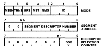
Figure 7. Control Registers
