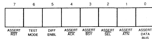
Figure 5.1: Initiator Command Register - Register Write
