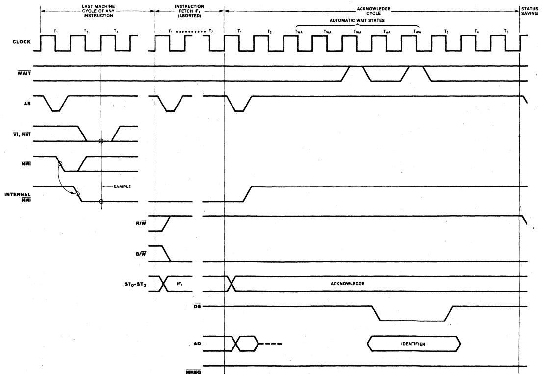
Figure 14. Interrupt and Segment Trap Request/Acknowledge Timing
