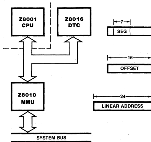
Figure 6. DTC Configurations
