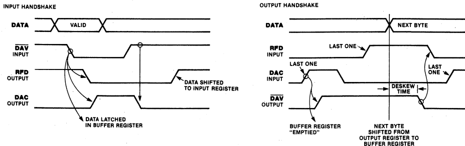
Figure 8. 3-Wire Handshake
