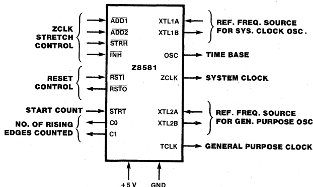
Figure 1. Pin Functions
