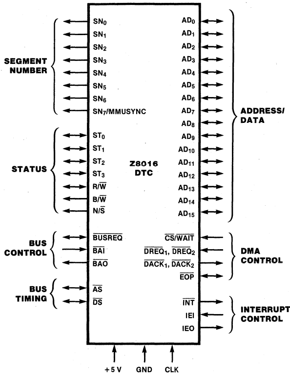
Figure 1. Pin Functions
