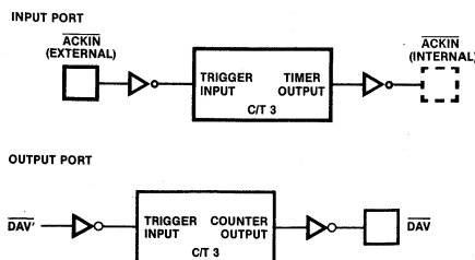
Figure 9. Pulsed Handshake
