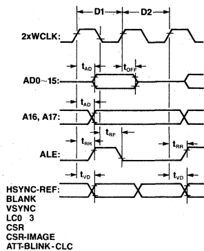
Display Memory Display Cycle Timing
