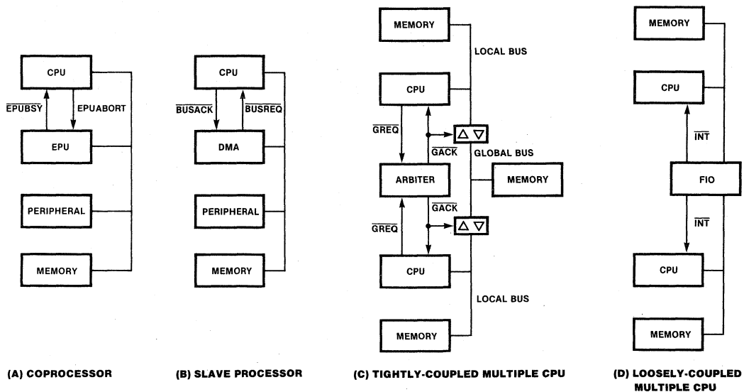
Figure 14. Multiprocessor Configurations
