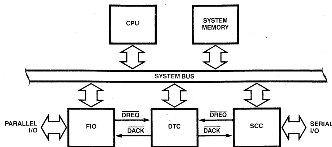
Figure 2. DTC Configuration
