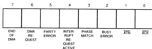
Figure 10.0: Bus and Status Register
