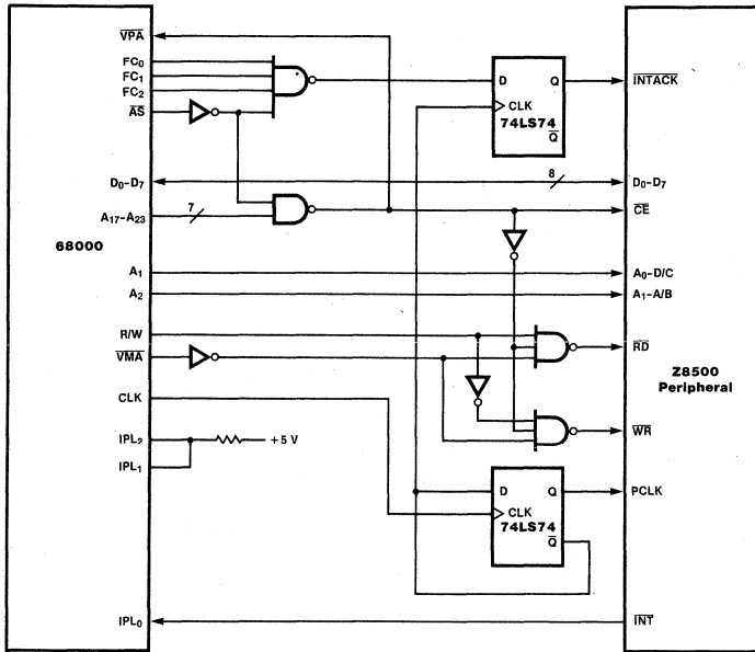
Figure 4. Interface Using the \overline{VPA} Cycle
