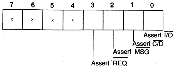
Figure 27.0 Register Reference Chart
