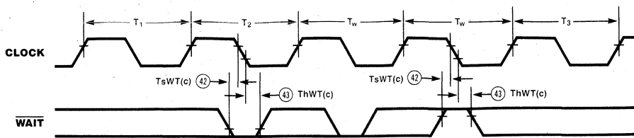
Figure 18. \overline{WAIT} Timing
