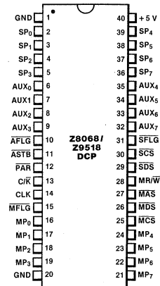
(DIP) Pin Assignments
