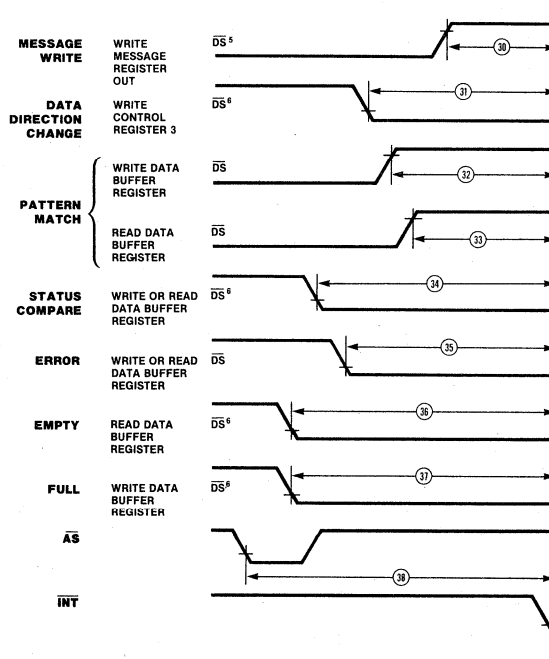
Figure 38. Z-BUS Interrupt Timing
