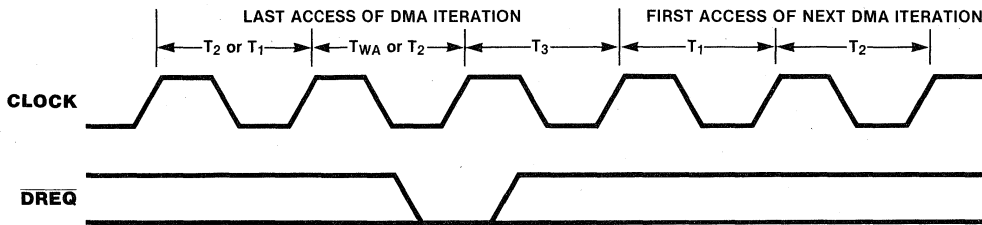
(B) \overline{DREQ} Sampling in Demand Mode During DMA Operations
