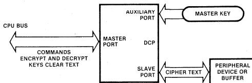
Figure 5a. Dual-Port Configuration, Multiplexed Control
