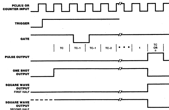
Figure 10. Counter/Timer Waveforms
