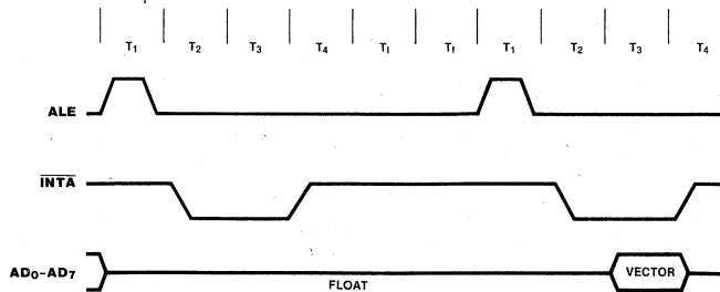
Figure 8. 8086/8088 INTA Sequence
