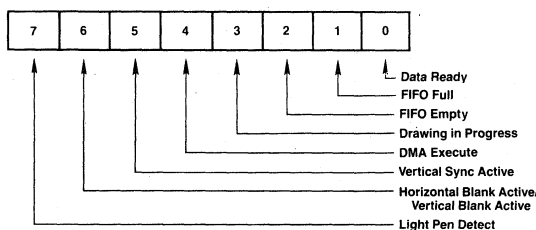
Status Register (SR)
