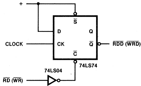
Figure 4. Delaying \overline{RD} or \overline{WR}
