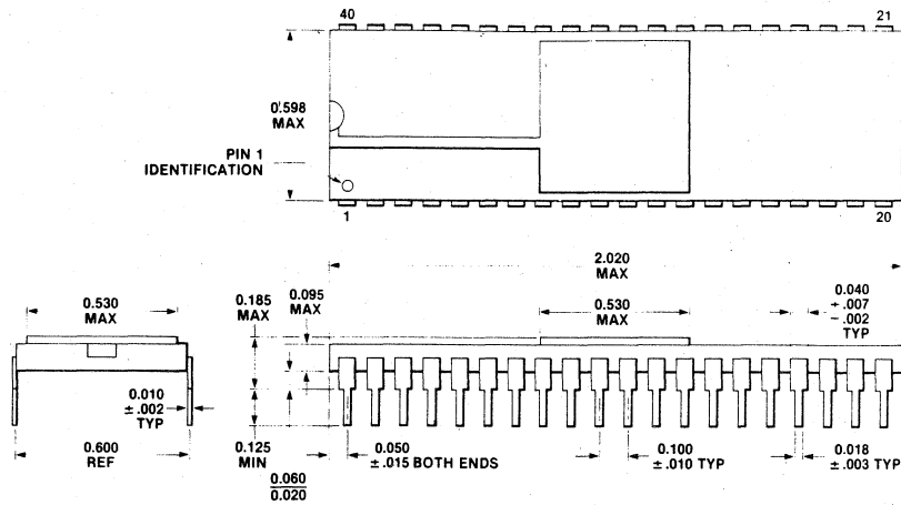
40-Pin Dual-in-Line Package (DIP), Ceramic
