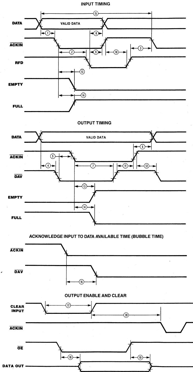
Figure 9. Timing Diagrams
