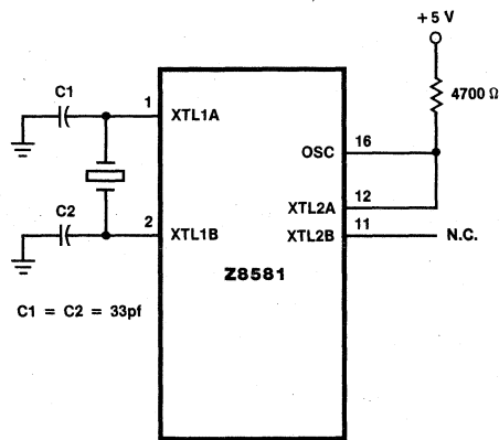
Figure 7. Circuit Configuration for Z8581
