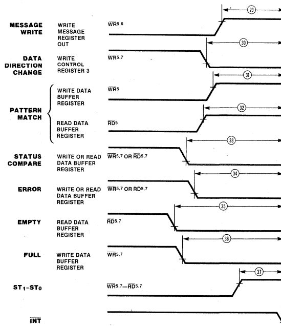
Figure 44. FIO Non-Z-BUS Interrupt Timing
