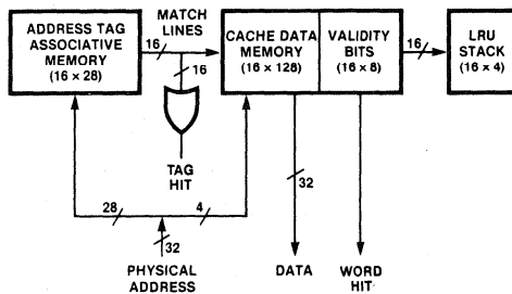
Figure 2. Cache Organization
