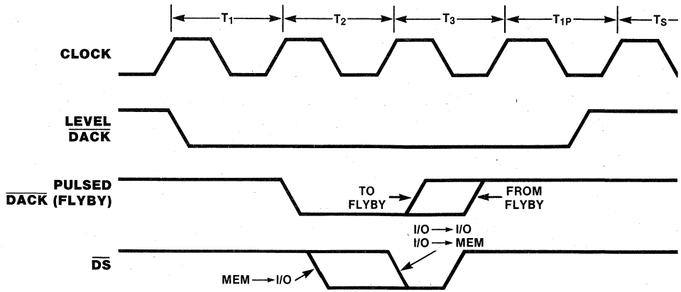
Figure 18. \overline{\text{DACK}} Timing
