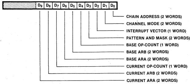
Figure A3. Chain Control Register
