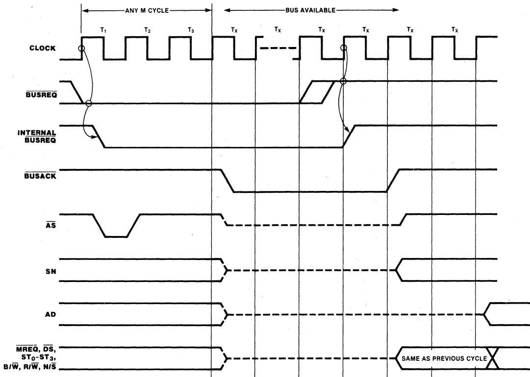
Figure 15. Bus Request/Acknowledge Timing
