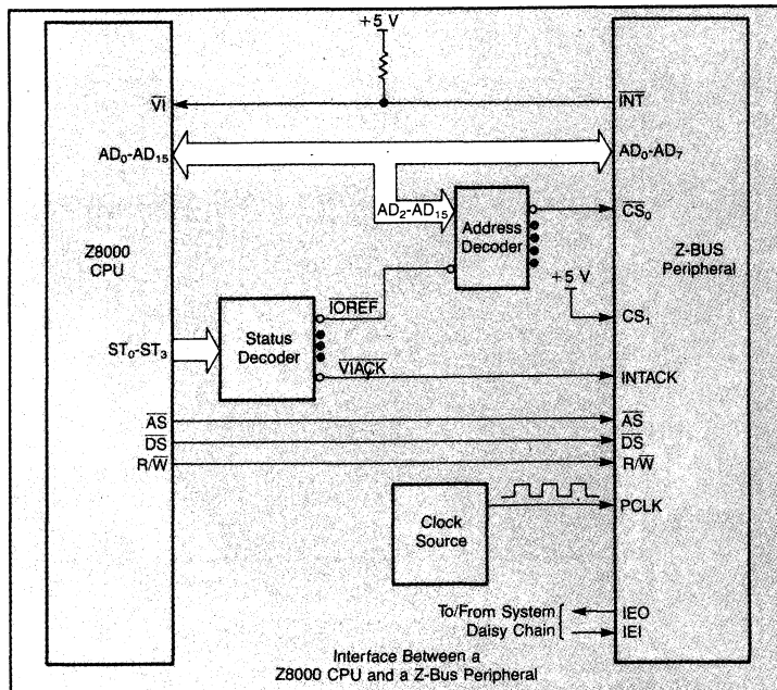
Figure 1: Interface between a Z8000 CPU and a Z-Bus peripheral.
