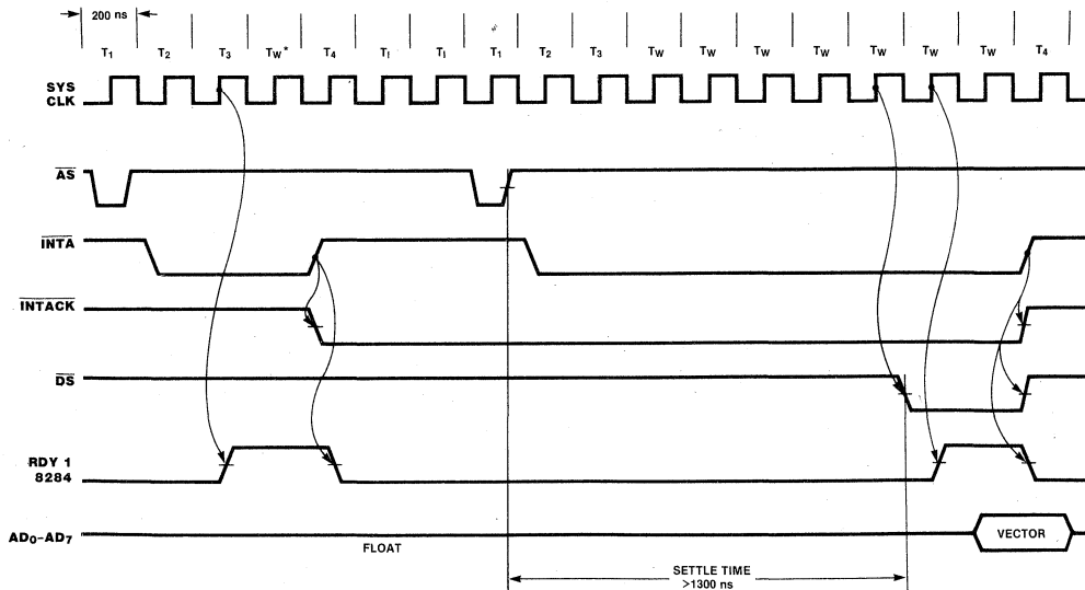
Figure 10. Interrupt Acknowledge Timing
