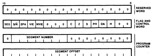
Z08001/Z160 Program Status Registers
