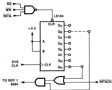
Figure 6. Multiple Wait State Generator
