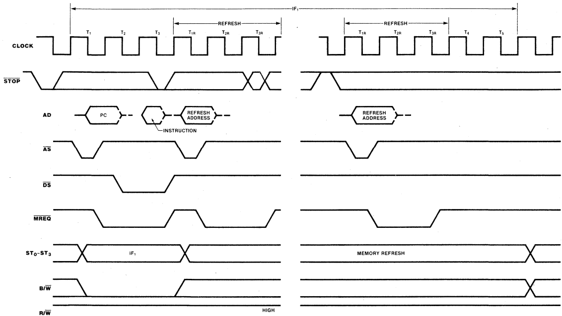
Figure 16. Stop Timing
