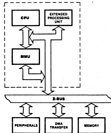
Figure 1. Z-BUS Connects All Functions
