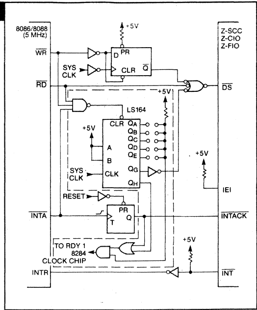
▲ Figure 5: Single wait state generator.
