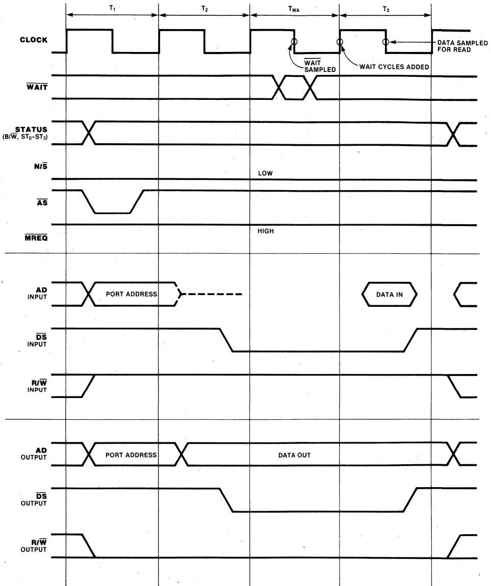
Figure 13. Input/Output Timing
