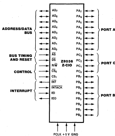
Figure 1. Pin Functions
