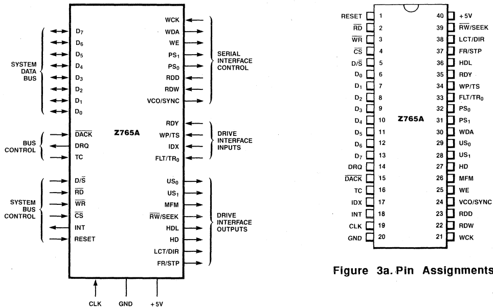
Figure 2. Pin Functions
