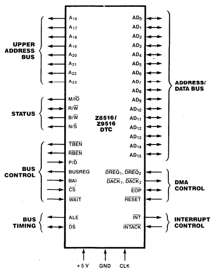
Figure 3. Pin Functions
