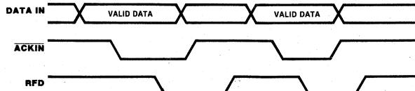
Figure 21. Interlocked Handshake Timing (Input) Port 2 Side Only
