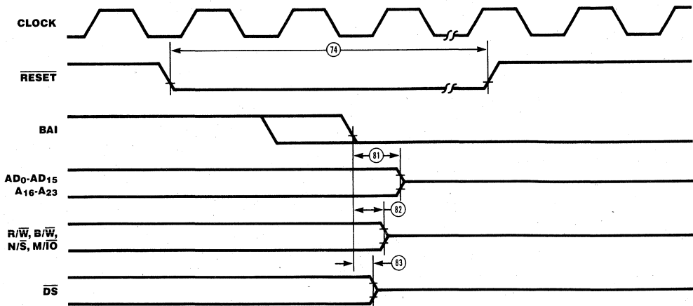
Figure 31. Reset Timing
