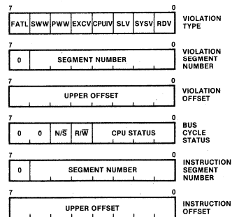
Figure 8. Status Registers
