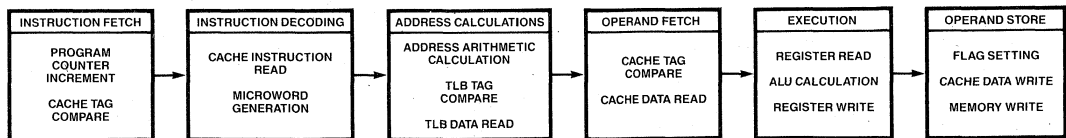
Figure 6. Instruction Pipeline
