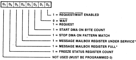
Figure 26. Control Registers
