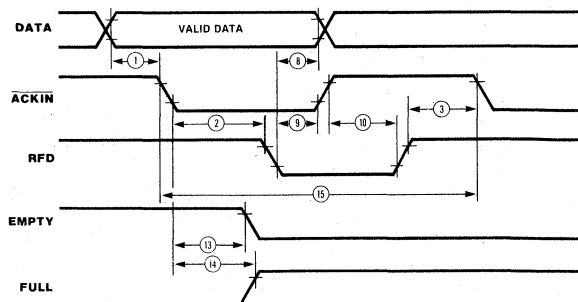
Figure 49. 2-Wire Handshake (Port 2 Side Only) Input
