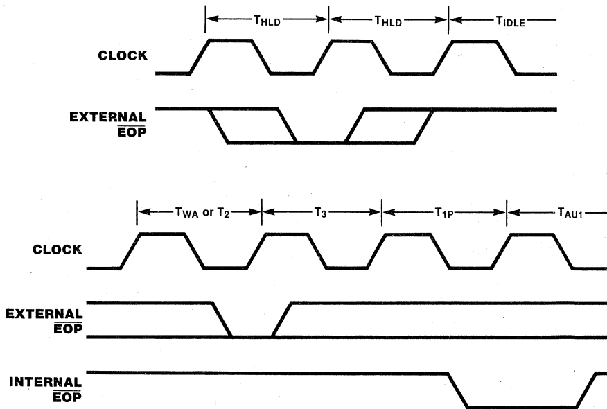
Figure 19. \overline{\text{EOP}} Timing
