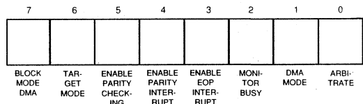
Figure 6.0: Mode Register
