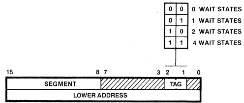
Figure 11. Chain Address Register
